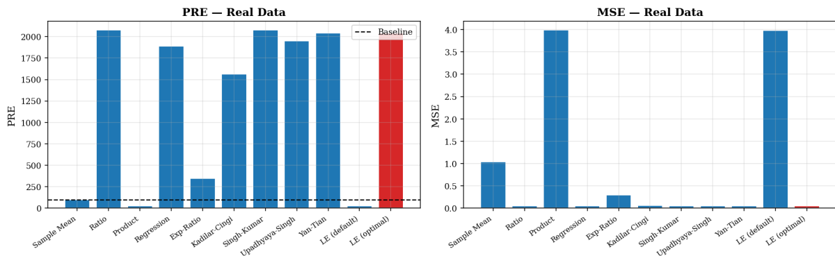
Figure 7: Figure 7: PRE and MSE of all estimators on the Murthy (1967) real dataset ( N = 50 , n = 20 ). The exceptionally high correlation ( \rho = 0.976 ) yields PRE values exceeding 2,000 for the best estimators.
