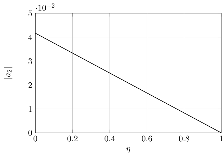
Figure 1: Variation of |a_2| with respect to \eta for fixed \lambda = 1 , \nu = 0.5 , n = 2 .
