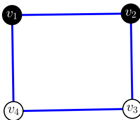
FIGURE 2. G(V, E)
