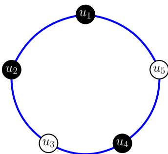
FIGURE 1. In this graph C_5 , D_f = \{u_1, u_2, u_4\} is a dominating set as well as a zero forcing set and no subset of the vertex set with cardinality less than three has this property, so F_d(C_5) = 3
