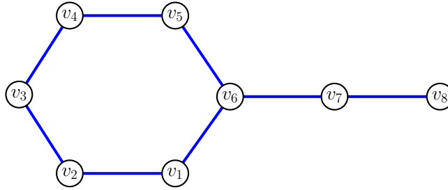
FIGURE 8. Graph for Example 5.14.
