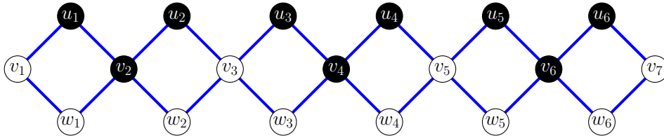
FIGURE 5. The Diamond Snake Graph D_6 . Dom-forcing set D_f = \{u_1, u_2, \dots, u_6, v_2, v_4, v_6\} and F_d(D_6) = 9
