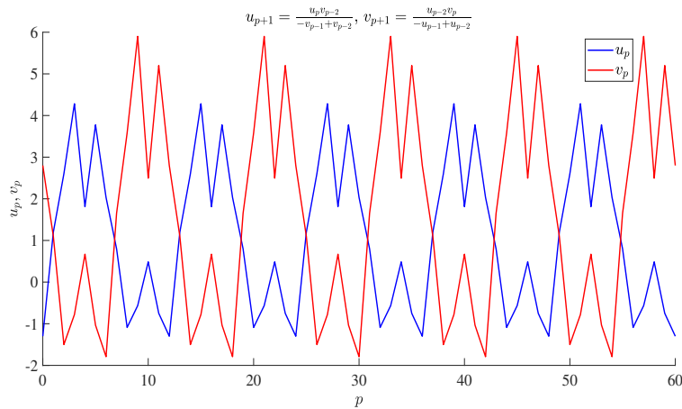
FIGURE 4. Numerical simulations for System (5.1) where x_{-2} = -1.3, x_{-1} = 1.2, x_0 = 2.6, y_{-2} = 2.8, y_{-1} = 1.1, y_0 = -1.5
