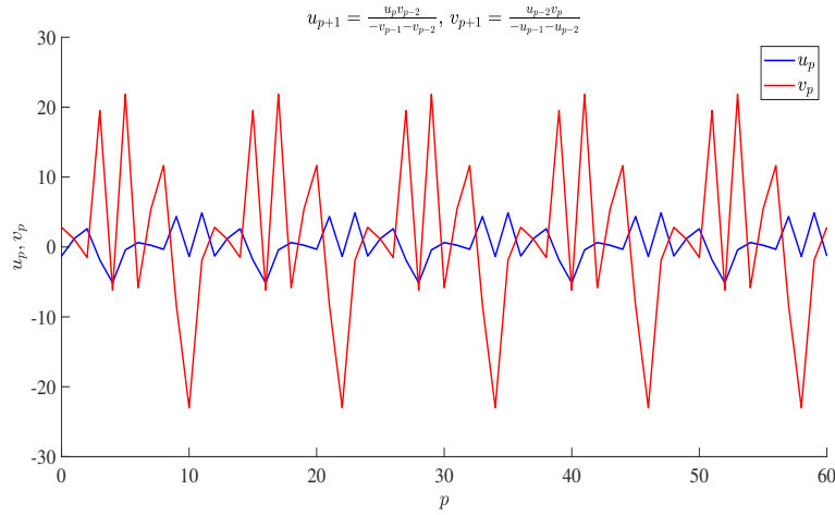
FIGURE 1. Numerical simulations for System (2.1) where x_{-2} = -1.3, x_{-1} = 1.2, x_0 = 2.6, y_{-2} = 2.8, y_{-1} = 1.1, y_0 = -1.5
