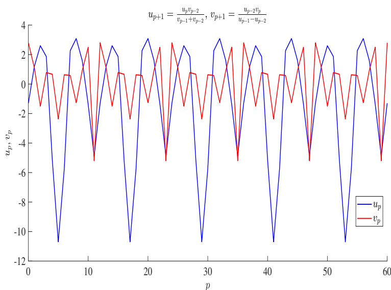
FIGURE 2. Numerical simulations for System (3.1) where x_{-2} = -1.3, x_{-1} = 1.2, x_0 = 2.6, y_{-2} = 2.8, y_{-1} = 1.1, y_0 = -1.5
