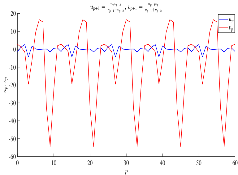
FIGURE 3. Numerical simulations for System (4.1) where x_{-2} = -1.3, x_{-1} = 1.2, x_0 = 2.6, y_{-2} = 2.8, y_{-1} = 1.1, y_0 = -1.5
