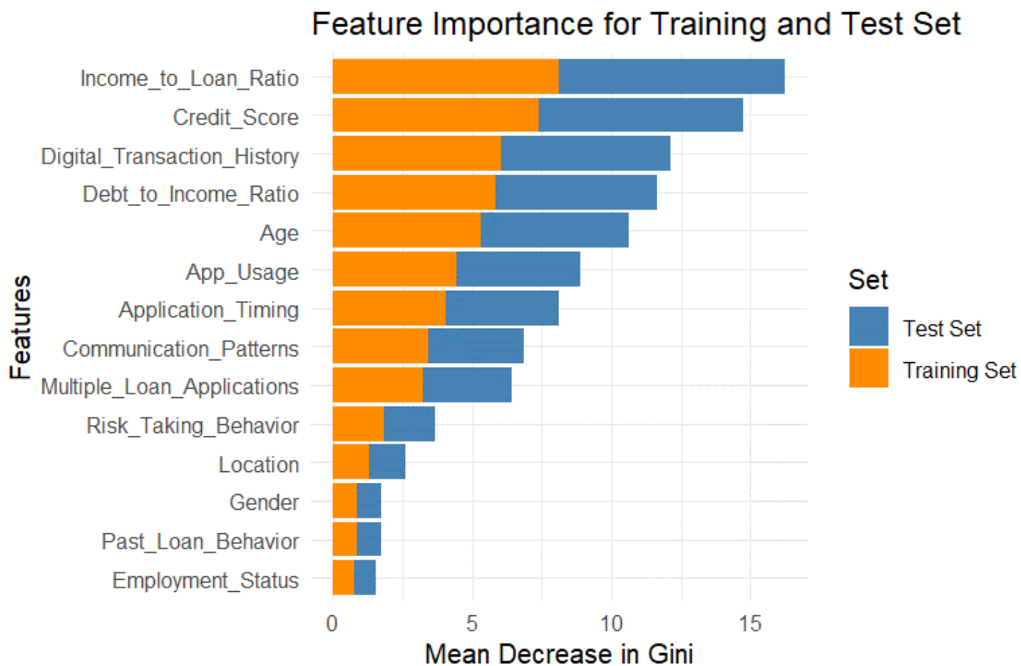
Figure 6: Feature Importance Combined
