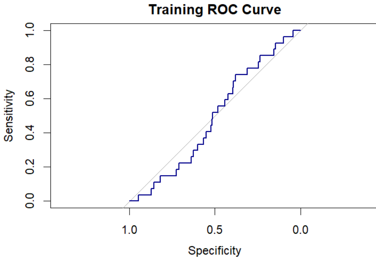
Figure 10: AUC-ROC Curve
