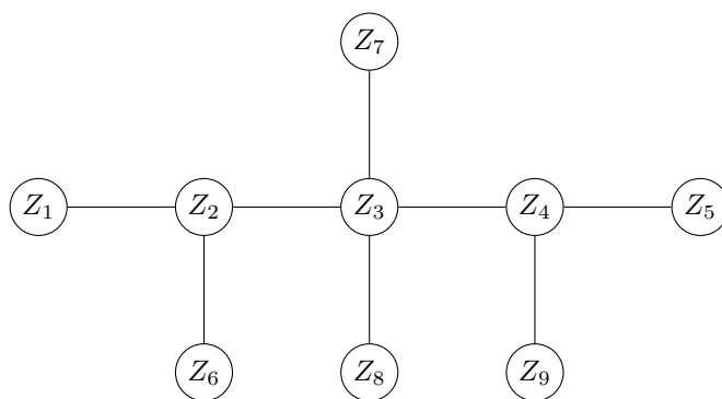
Graph 2. Molecular graph of first Zagrab index
