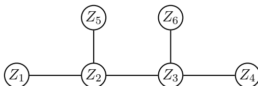
Graph 1. Eccentricity of first Zagrab index
