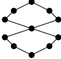
FIGURE 1. S(P_4)
