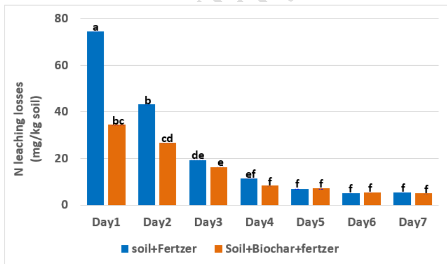
Figure 2. Daily leaching losses of nitrogen in the presence of fertilizer application for control soil without biochar and soil treated with biochar
