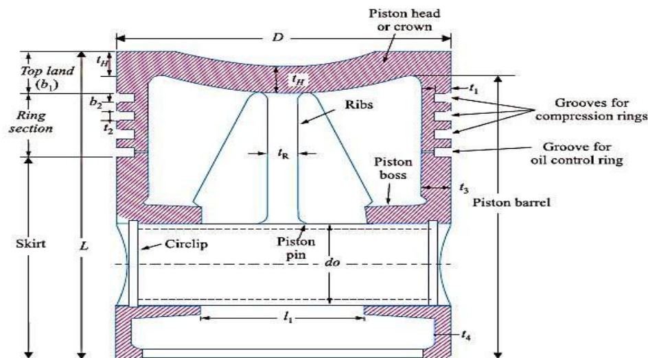
Figure 1: Section of Piston for I.C. engines (Khurmi and Gupta, 2007) [2]
