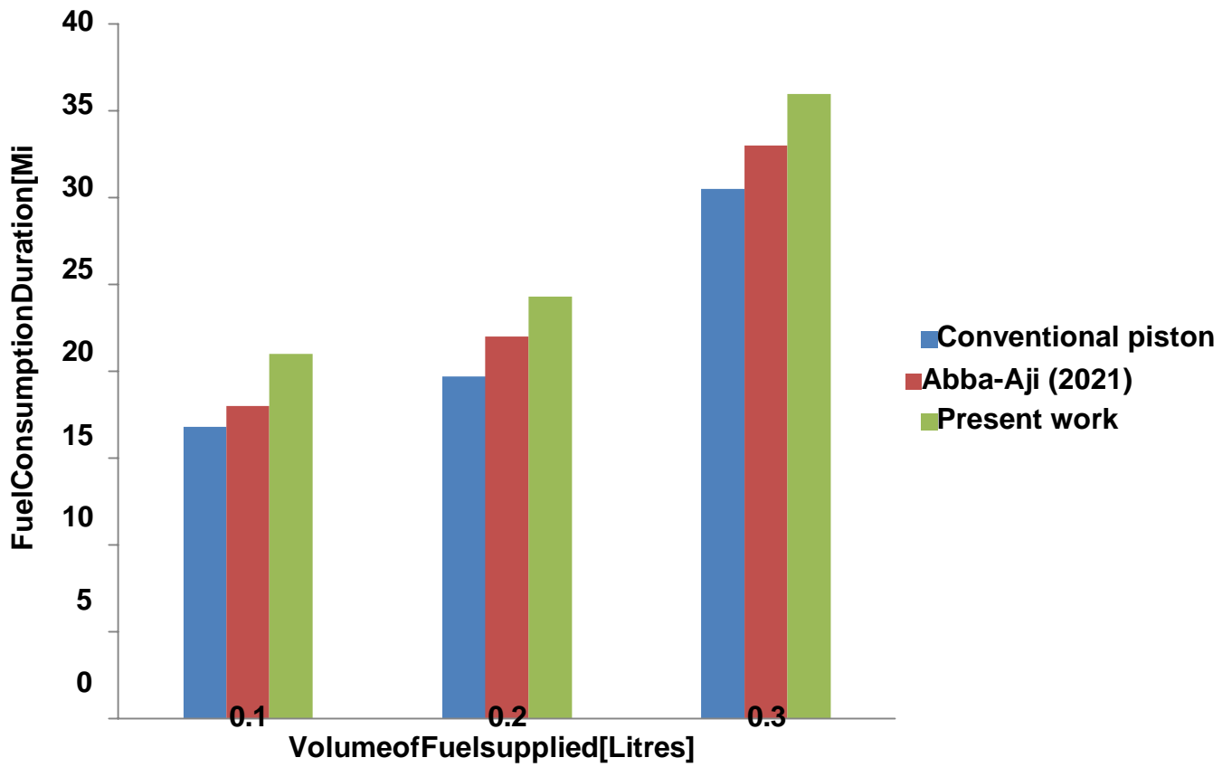
Figure 6: Engine fuel consumption duration
