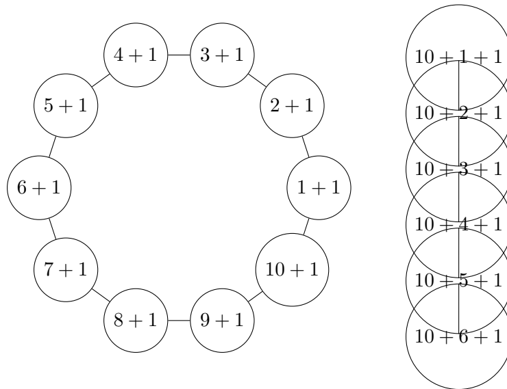
Figure 5: Generalized structure of C_{10} \cup P_6 with Fibonacci labeling
