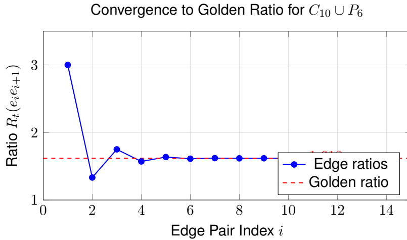
Figure 6: Convergence of edge label ratios for C_{10} \cup P_6
