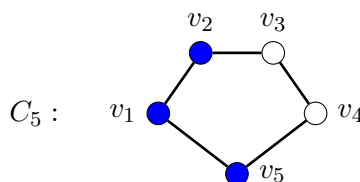
Figure 1: A restrained semitotal dominating set of V(C_5)
