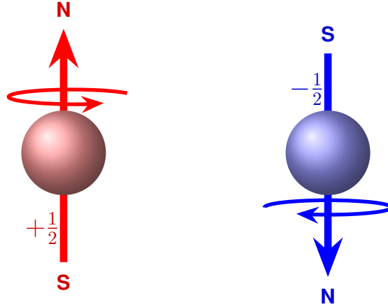
Figure 1: Angular Momentum \omega = Ec/\hbar
