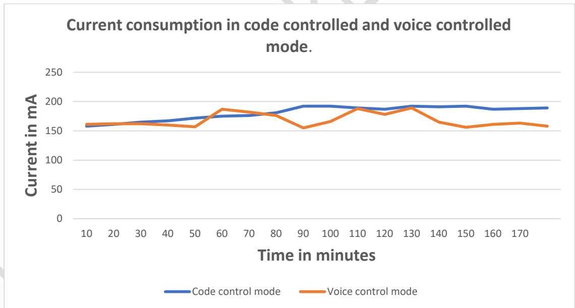
Graph 2: Current consumption of DHT11 sensor in code-controlled and voice-controlled mode of operation.
