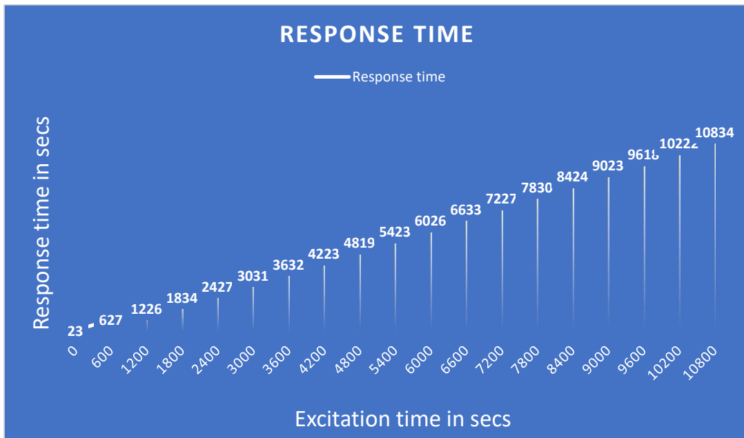
Graph 3: Time delay between excitation and response of DHT11 sensor in voice-controlled mode.
