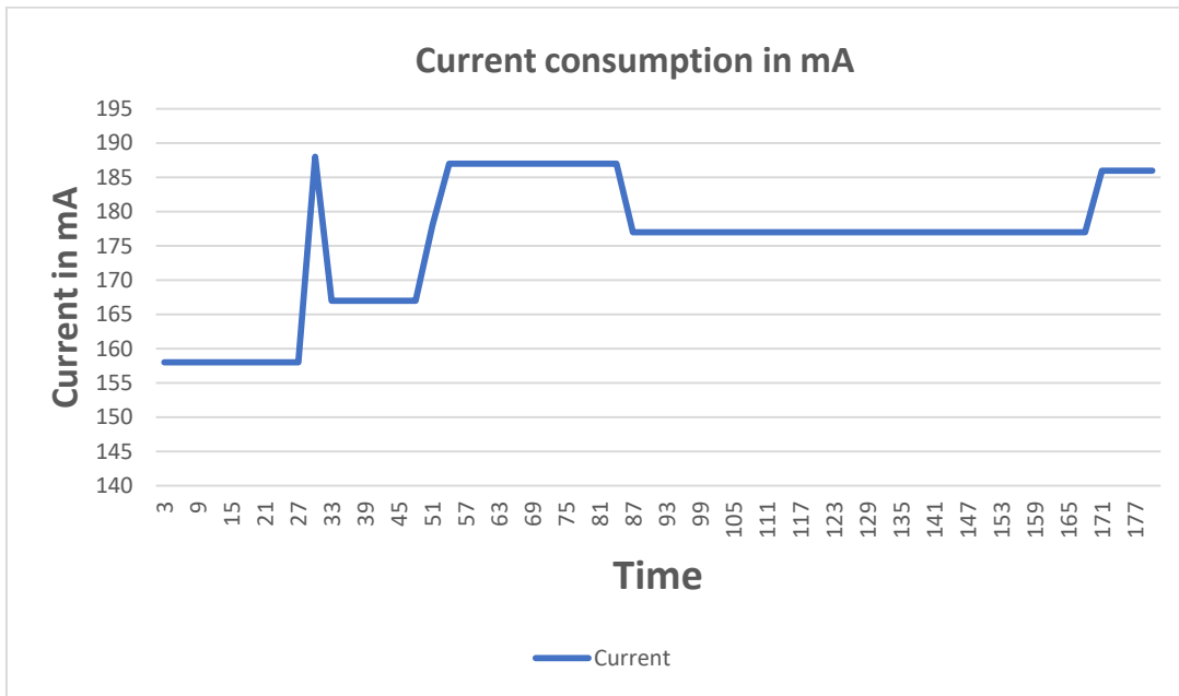
Graph 1: Current consumption of DHT11 sensor in continuous operation.
