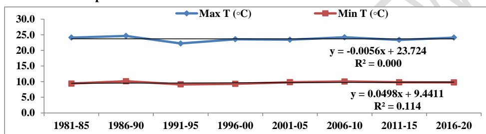
Figure 11: Pentadal trend analysis of maximum and minimum temperature in the Rabi season for plain zone of Uttarakhand
