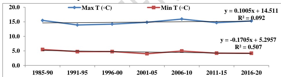
Figure 12: Pentadal trend analysis of maximum and minimum temperature in the Rabi season for hill zone of Uttarakhand
