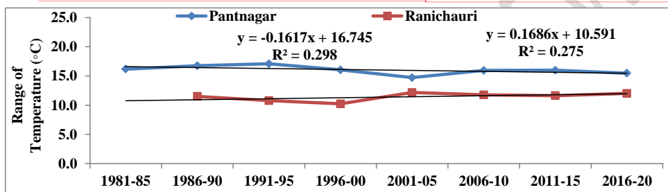
Figure 7: Pentadal trend analysis of range of temperature in the Zaid season for both the plain and hill zones of Uttarakhand
