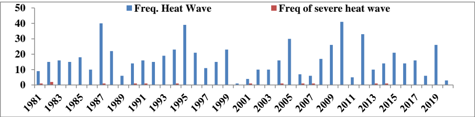
Figure 16: Frequency of heat waves in plain zone of Uttarakhand
