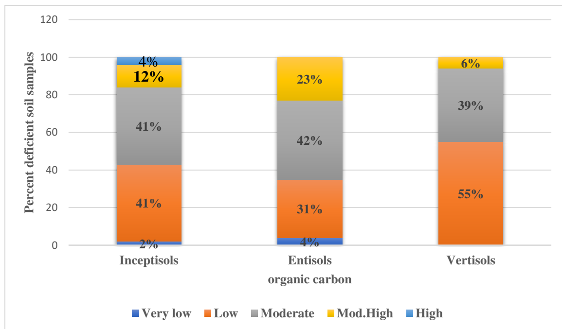
Fig. 1. Status of organic carbon in Inceptisols, Entisols and Vertisols
