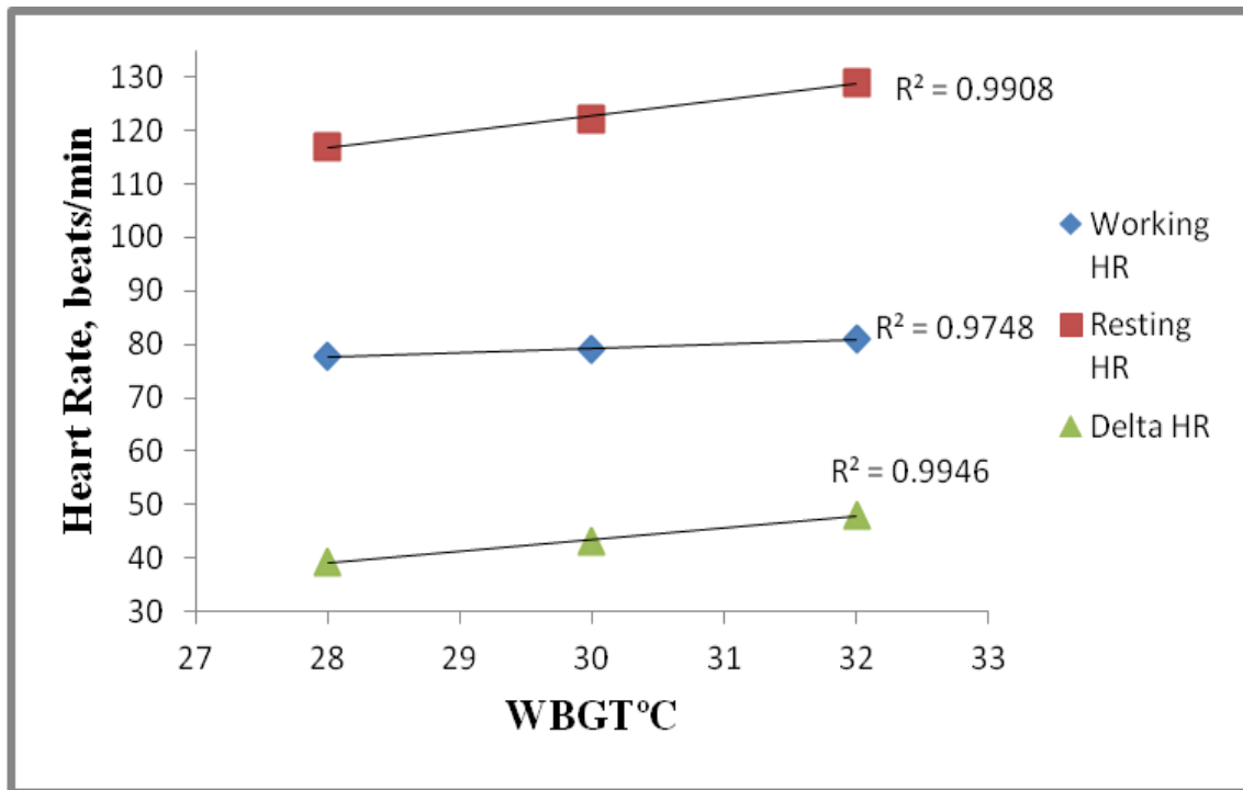
Fig. 2 Effect of WBGT on heart rate
