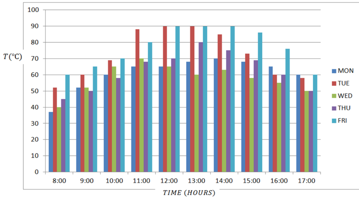
Figure 13: Temperature ( ^{\circ}\text{C} ) against time (hrs) for five days for water.
