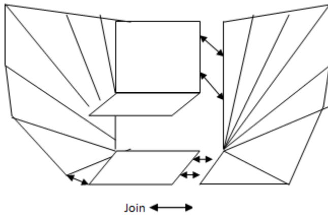
Figure 10 panel cooker in its box design
