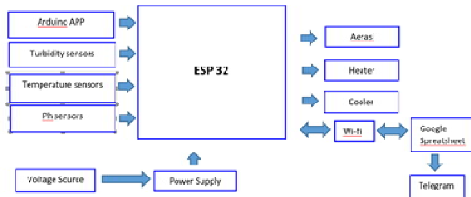
Figure 2. Block Diagram of IoT-Based Water Quality Control System
