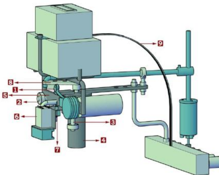
Figure 2 : The Schematic Diagram of the Designed Robot Weed Controlback view
