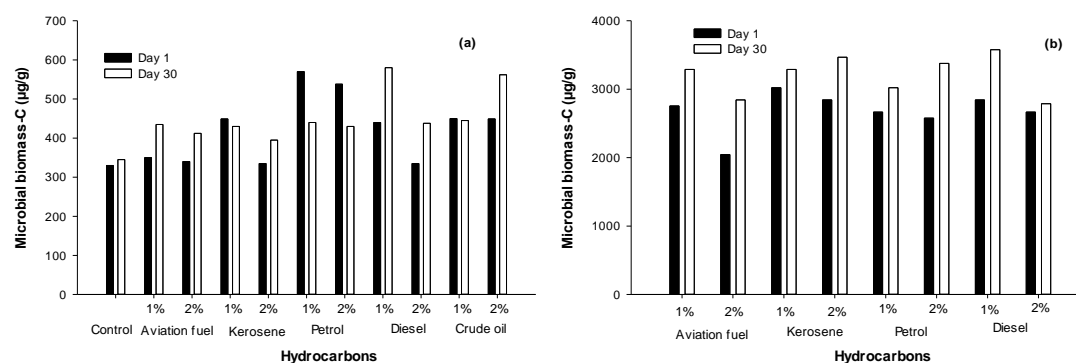
Figure 4: Soil microbial biomass-C ( \mu\text{g/g} soil) in (a) uncontaminated soil and HC-contaminated soils and (b) HC-contaminated soils amended with HC-adapted degraders at (■) 1 d and (□) 30 d of contamination
