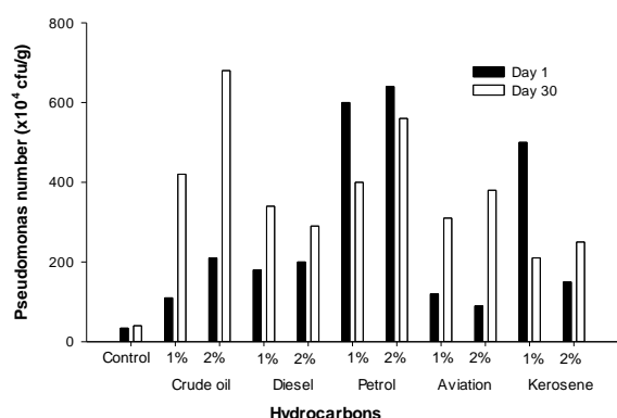
Figure 5: Populations (cfu.g -1 ) of PAH-degrading Pseudomonas sp. in uncontaminated soil and HC-contaminated soils at (■) 1 d and (□) 30 d of contamination
