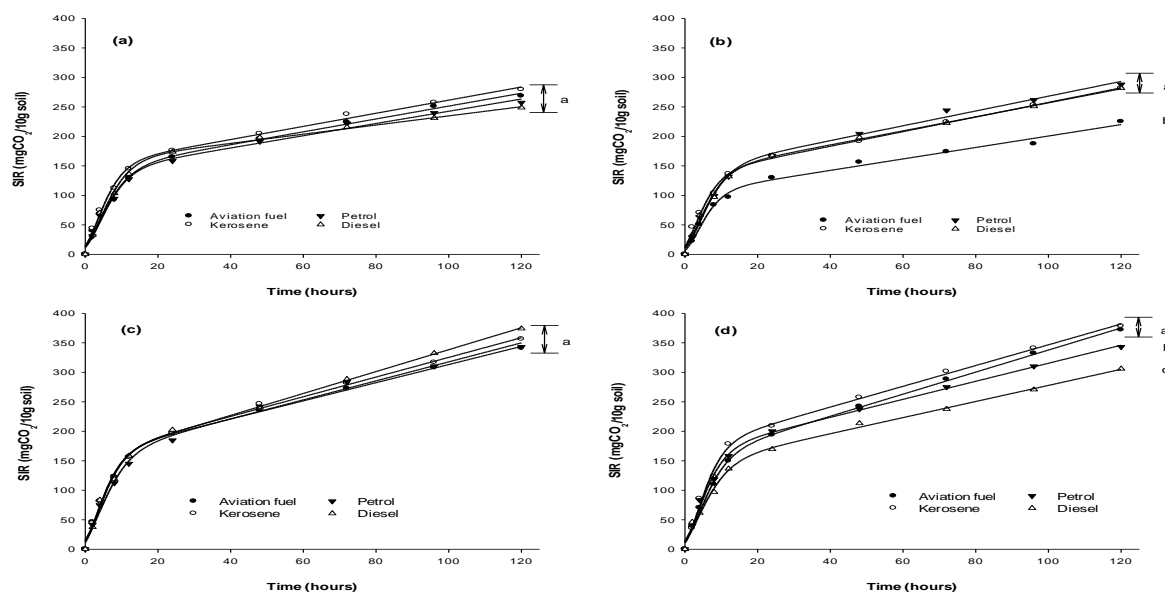
Figure 3: Substrate-induced respiration in HC-contaminated soils and amended with HC-adapted degraders (●) aviation fuel, (○) kerosene, (▼) petrol, and (Δ) diesel applied at (a) 1% w/w and (b) 2% w/w contaminant levels after 1 d and at (c) 1% w/w and (d) 2% w/w contaminant levels after 30 d of contamination
