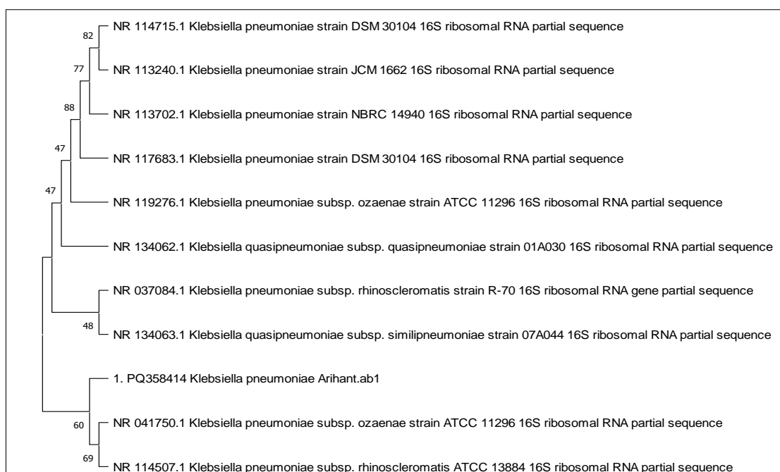
Fig 6: A phylogenetic tree based on 16S rRNA gene sequences
