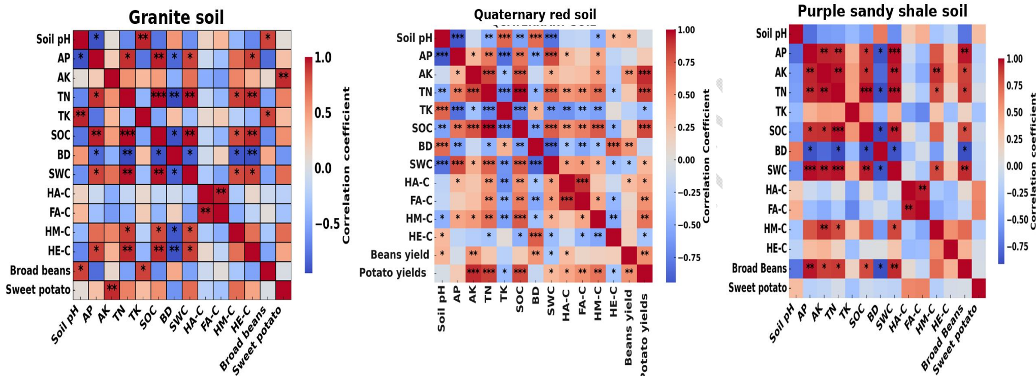
Figure 7. Correlation Analysis amongst soil properties, sweet potato ( Ipomoea batatas 'Beauregard') and broad bean ( Vicia faba 'Aquadulce Claudia') yields and soil humus carbon fractions in granite, Quaternary and purple sandy shale soils. (*) correlation is significant at the P < 0.05 level, (**) correlation significant at the P < 0.01 level, (***) correlation significant at the P < 0.001 level. BD (Bulk density), SWC (Soil water capacity), TN (Total nitrogen), AP (Available phosphorus), AK (Available potassium), TP (Total phosphorus), TK (Total potassium), SOC (Soil organic carbon), HA-C (Humic acids carbon), FA-C (Fulvic acids carbon), and HU-C (Huimin carbon).
