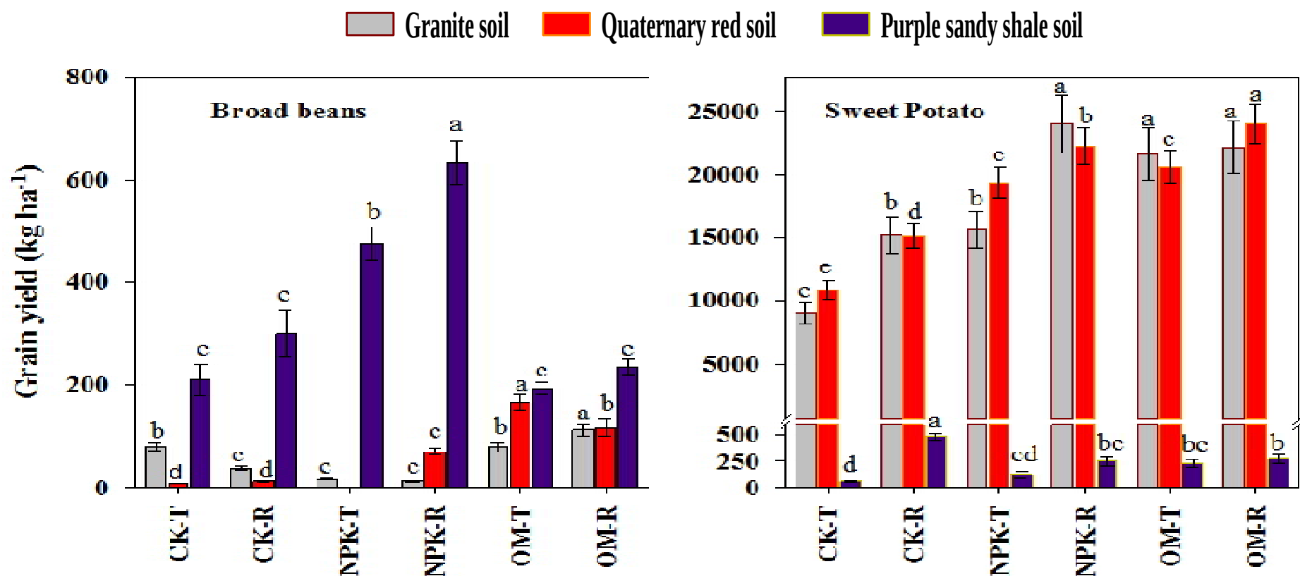
Figure 6. Sweet potato ( Ipomoea batatas 'Beauregard') and broad bean ( Vicia faba 'Aquadulce Claudia') yields under different long-term fertilization treatments in granite, Quaternary red soils and purple sandy shale soil. Lowercase letters indicate statistical significance ( P < 0.05 ) where different letters above the bars mean significant differences in yields among soil treatments.
