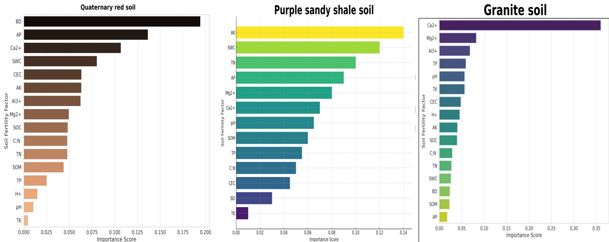
Figure 8. Relative importance of fertility factors in the granite, Quaternary red and purple sandy shale soils based on random forest model.
