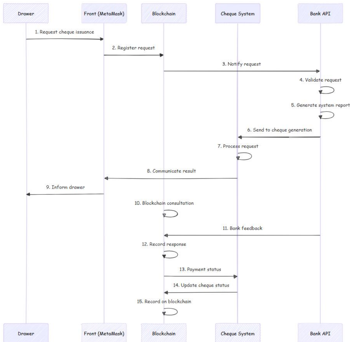
Fig. 7 Flow diagram of cheque generation process
