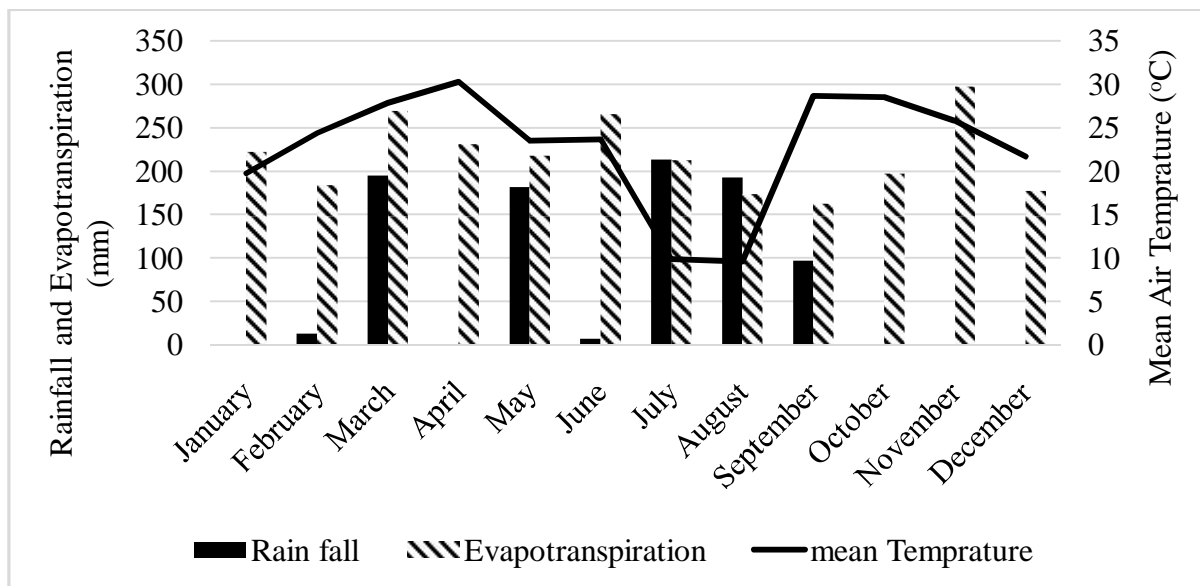
Figure 1 Mean annual rainfall, evapotranspiration and air temperature in the study area (January – December, 2017)
