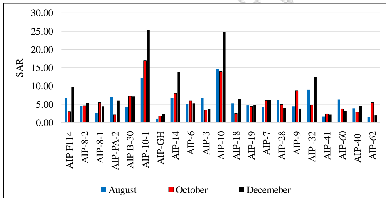
Figure 4 Temporal trend of soil SAR values at 0-30 cm soil depth in Fluvisols areas
