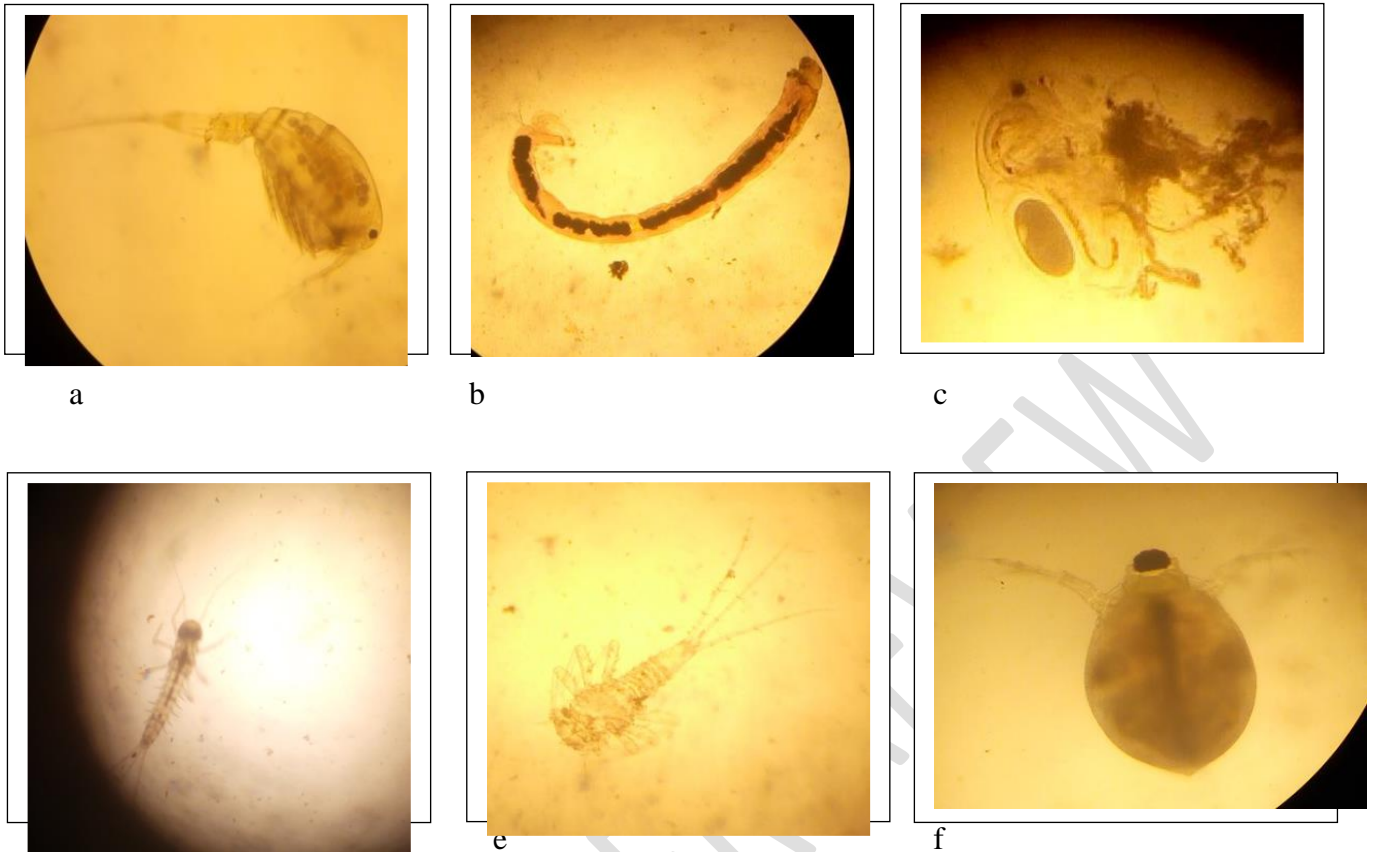
Figure 2: A Cross section of some identified zooplankton
