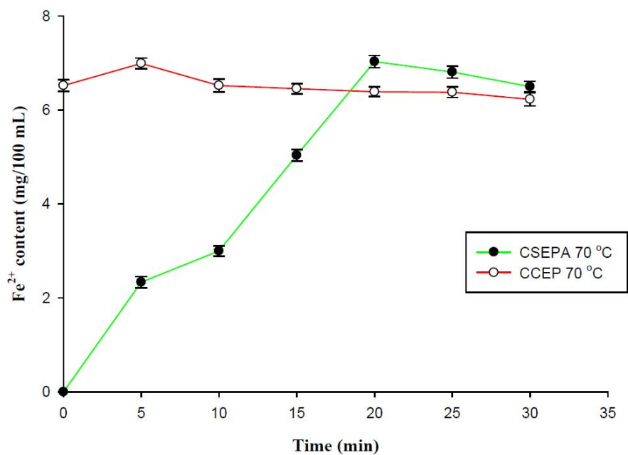
Fig. 6d. Comparison of \text{Fe}^{2+} content for CSEPA and CCEP at 70 °C
