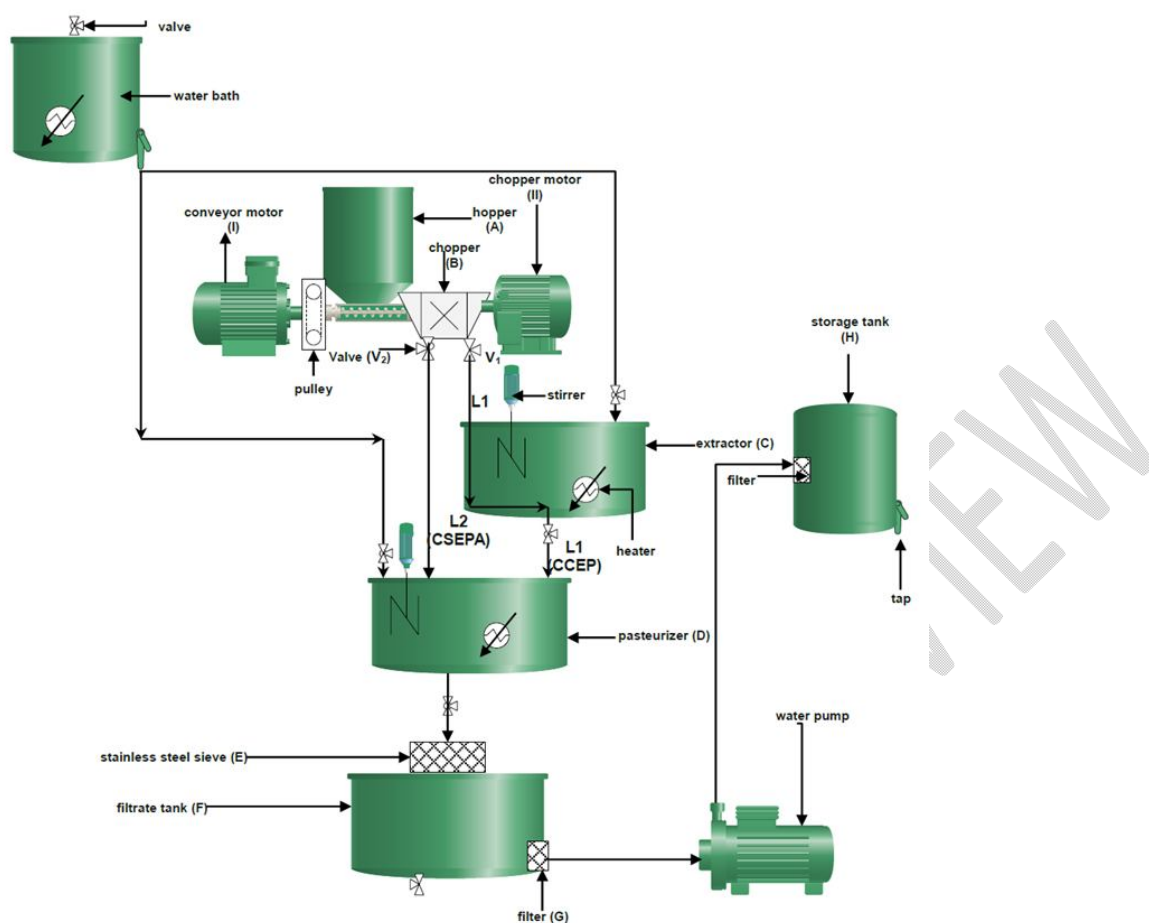
Fig.1. Flowsheet of the Developed Continuous Simultaneous Extraction and Pasteurizing system
