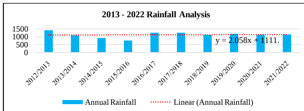
Figure 4C: 2013 – 2022 Rainfall analysis from Msekera weather station
