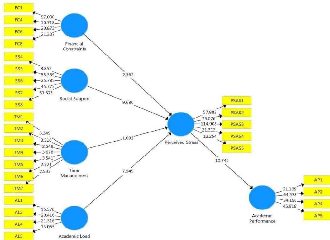
Figure2:PLSBootstrapping
