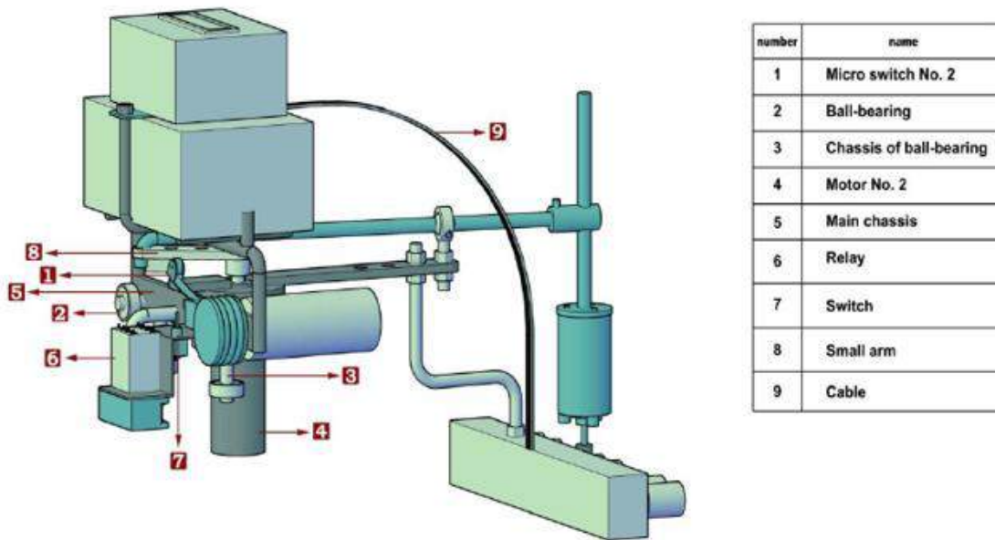
Figure 2 : The Schematic Diagram of the Designed Robot Weed Control back view
