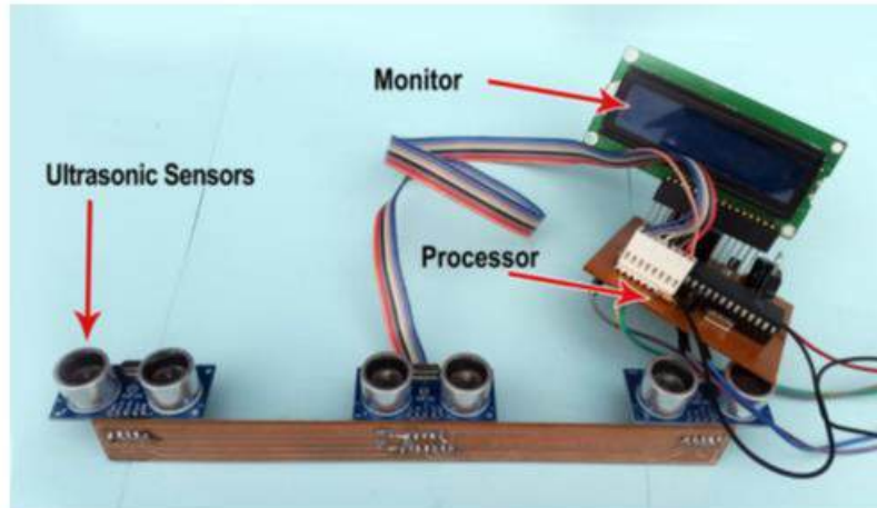
Figure 6 : Electronic modules of the robot
