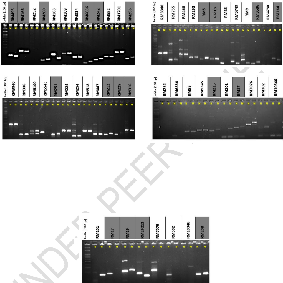
Figure 1: Amplification profile of polymorphic markers. The labels in grey denote polymorphic markers and white denotes monomorphic markers.
