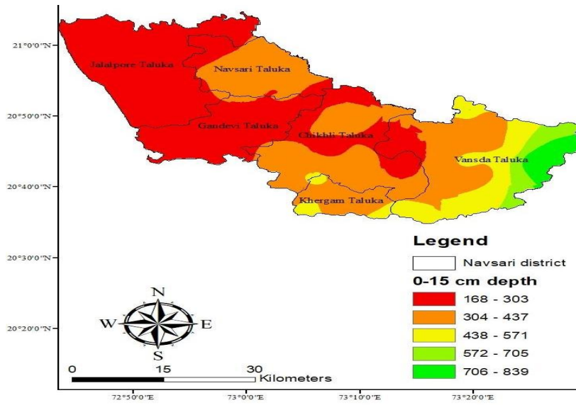
Fig. 2:- Available Nitrogen (kg/ha) status at 0-15 cm depth
