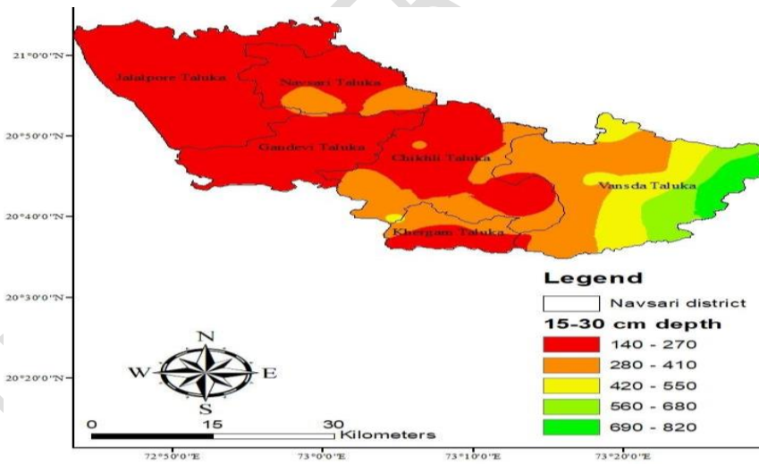
Fig. 3:- Available Nitrogen (kg/ha) status at 15-30 cm depth
