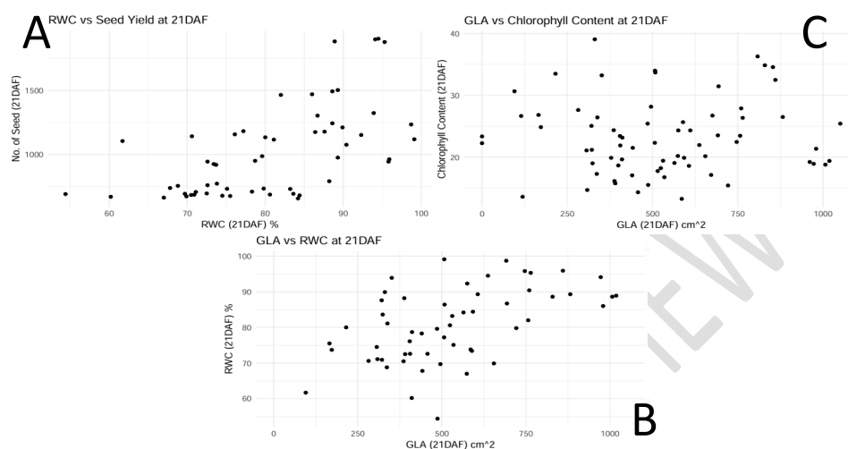
Figure 1: Scatter plot depicting relationships among variables
