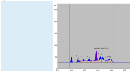
Figure 1a. Typical Chromatogram of standard ursolic acid
