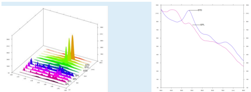
Figure 2. 3D spectra of Ursolic acid + B.racemosa Figure 3. Spectral comparison of Standard Ursolic acid and B.racemosa
