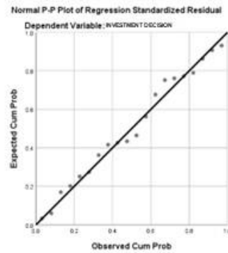
Figure 2. Normality Test 2
