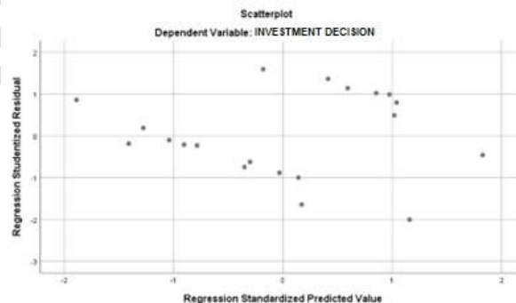
Figure 3. Heteroscedasticity Test
