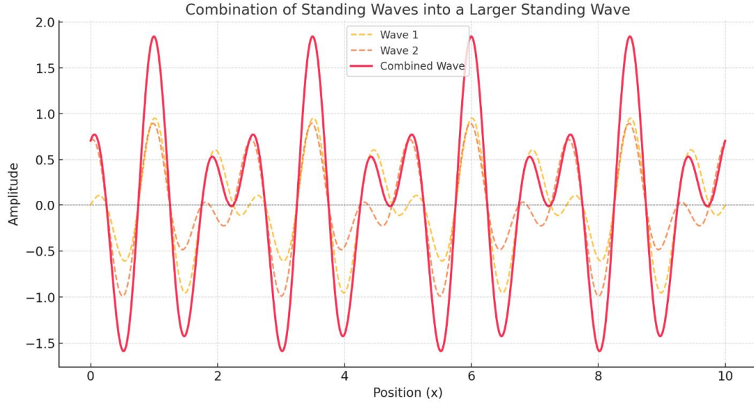
Figure 2: Interaction of two standing waves with a slight phase difference demonstrates how constructive and destructive interference leads to the formation of a larger, more complex standing wave. This process illustrates the principles of self-organization and coherence in oscillatory systems, as seen in the scalar field framework, where overlapping toroidal waves combine to create emergent physical structures.
