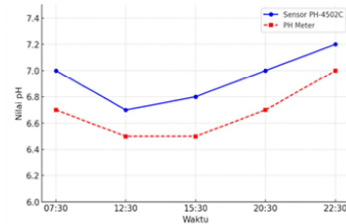
Figure 9 Test results of the PH-4502C sensor with a PH meter
