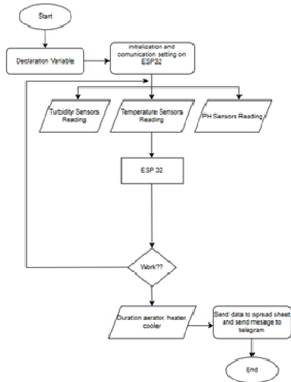
Figure 4. Flowchart of IoT-Based Water Quality Control System
