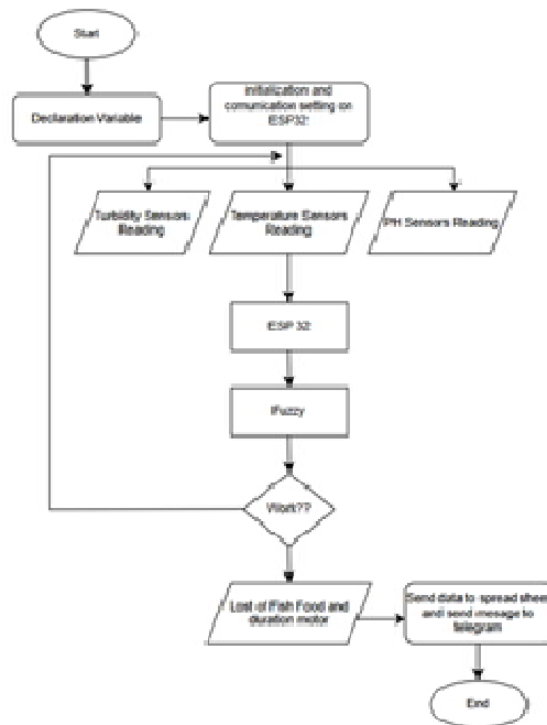
Figure 5. Flowchart of IoT and Fuzzy Based Fish Feeding System
