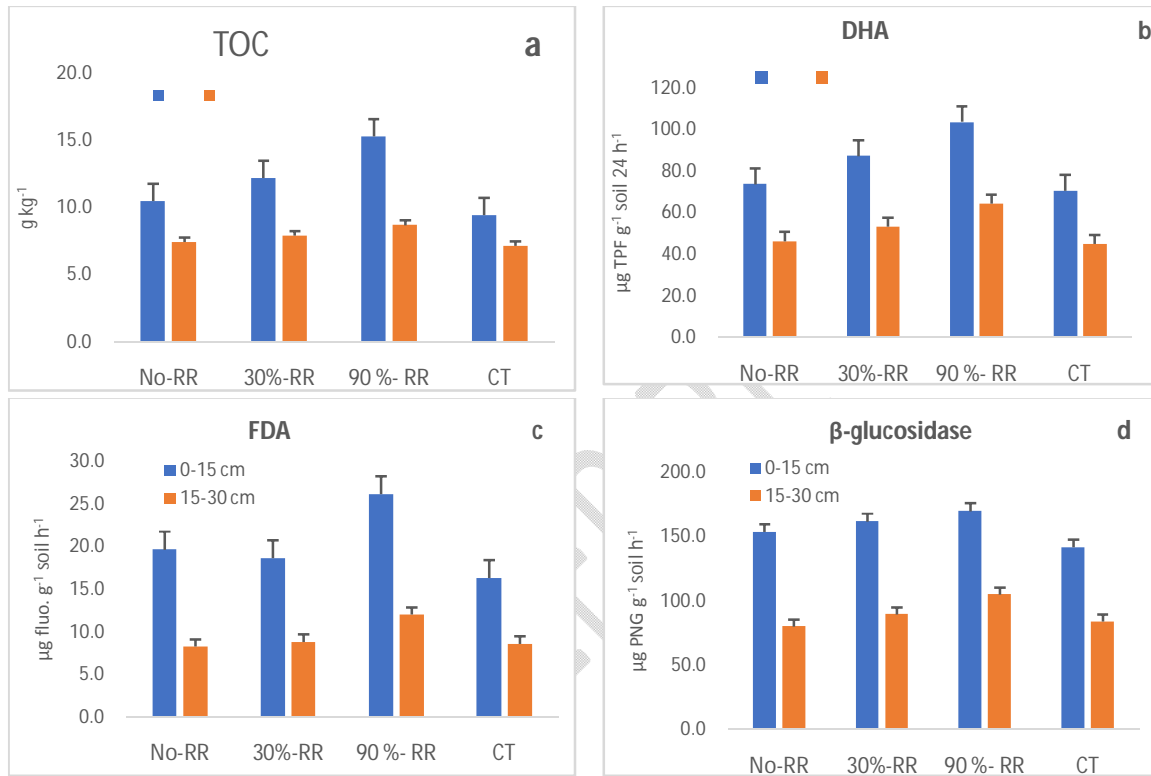
Figure 1. Total organic carbon (TOC) in soil samples collected from fields under different residue retention and tillage practices. Soil enzymatic activities (b) DHA, (c) FDA, (d) \beta -glucosidase were estimated under different residue retention (RR) and conventional tillage at the different depth 0-15 cm and 15-30 cm. The residue retentions are no residue retention (0%), 30% residue retention and 90% residue retention. Each data point represents average with error bar as standard error of three replicated observations. Significant difference between treatments was indicated with p < 0.05 .
