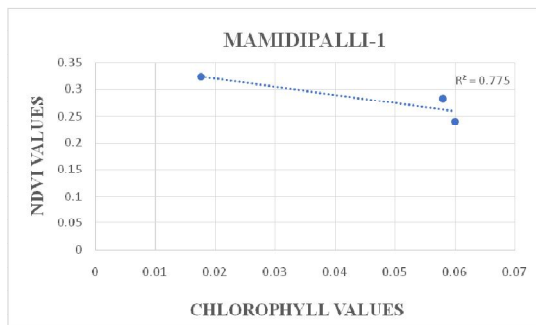
Fig:3Correlation between Chlorophyll and NDVI values of Landsat 8 Satellite Images.
