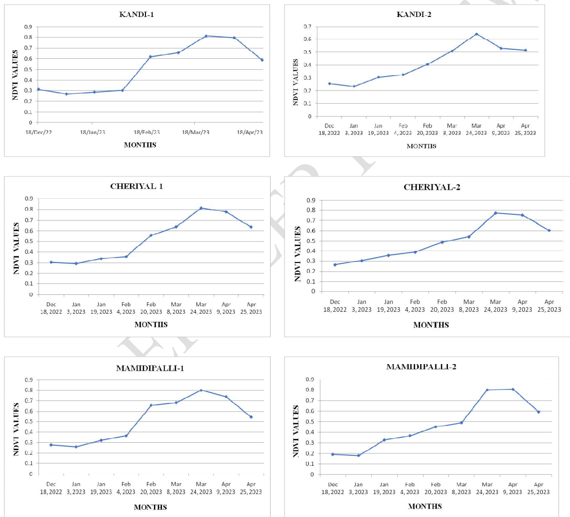
Fig:7 NDVI trend of six location in Kandi Mandl using Landsat-8 Satellite
