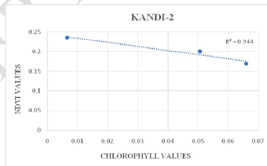
Fig:3Correlation between Chlorophyll and NDVI values of Landsat 8 Satellite Images.
