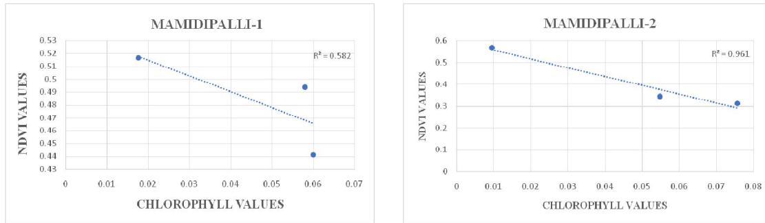
Fig:4 Correlation between Chlorophyll and NDVI values of Semtinel-2 Satellite Images.
