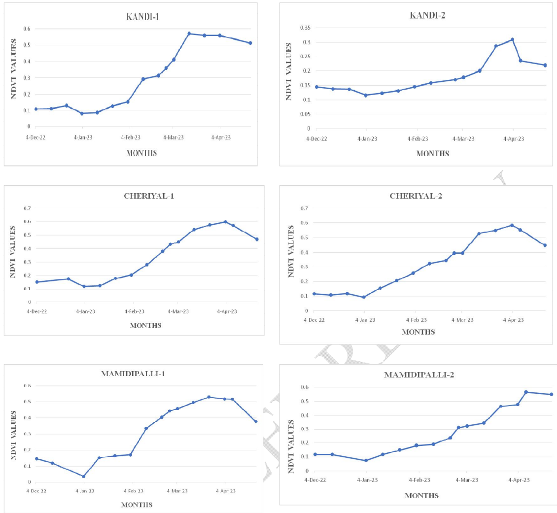
Fig:8 NDVI trend of six location in Kandi Mandl using Sentinel-2 Satellite
