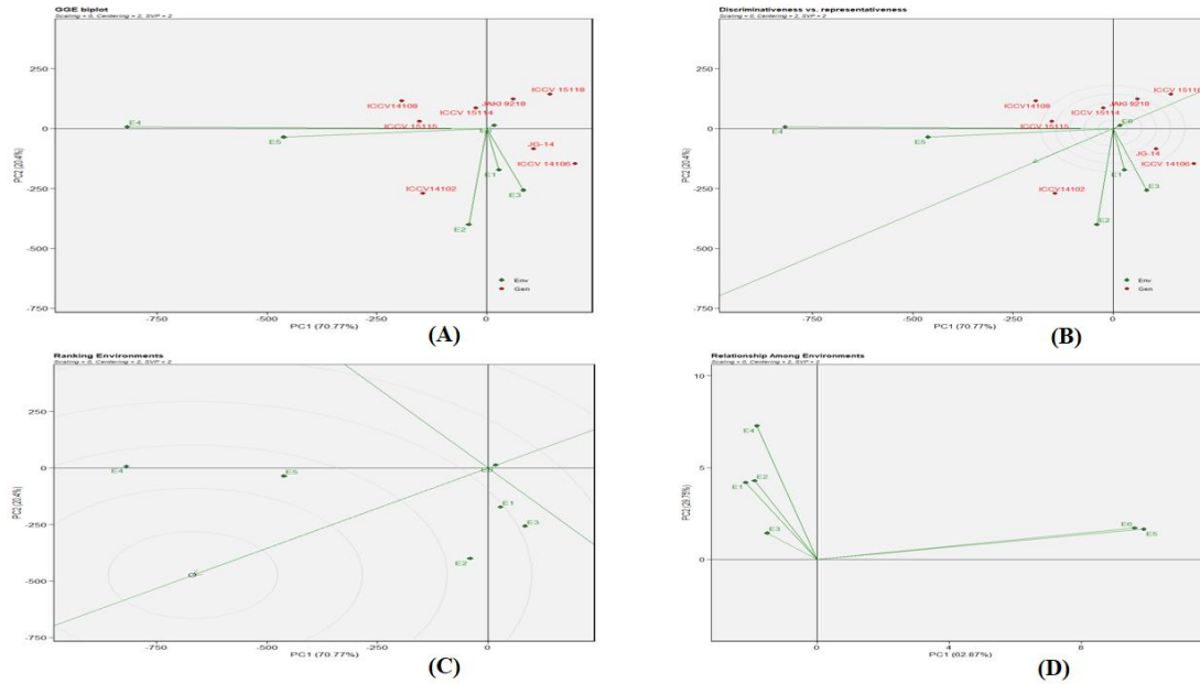
Figure-1: GGE Biplot analysis (A) GGE biplot; (B) Discriminateness Vs representativeness; (C) Ranking environment; and (D) Relationship among environment
