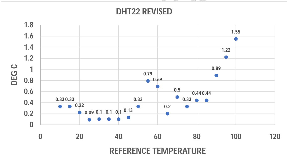
Graph 11: Absolute error of DHT22 with second method.
