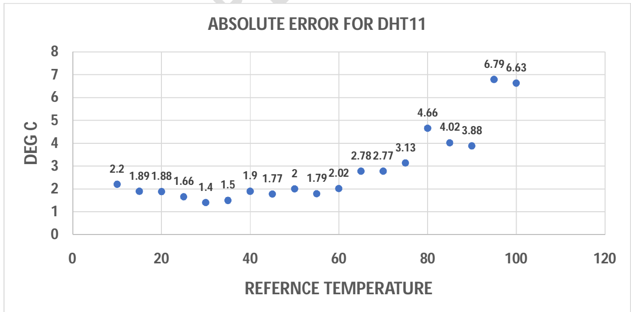
Graph 1. Absolute error of DHT11 with first method
