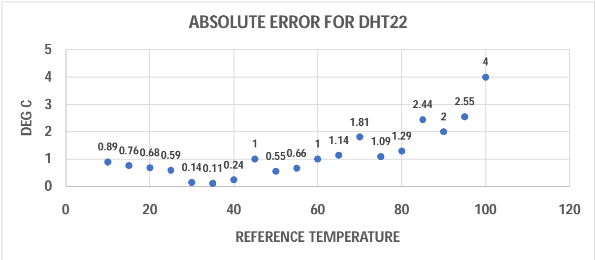
Graph 2: Absolute error for DHT22 with first method.
