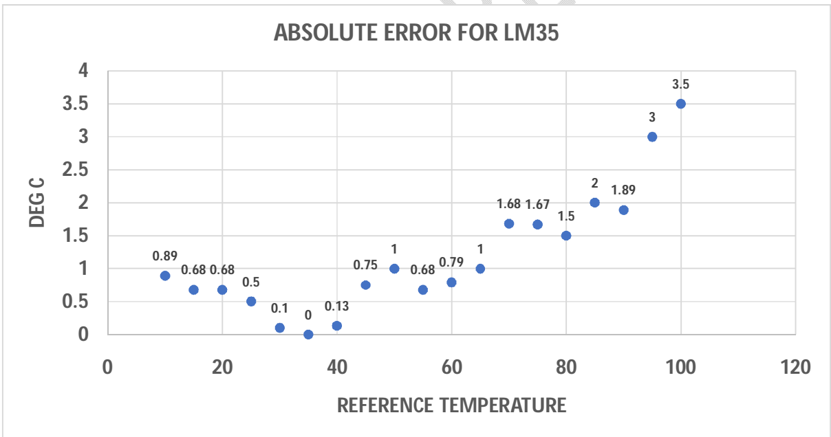
Graph 3: Absolute error for LM35 with first method.
