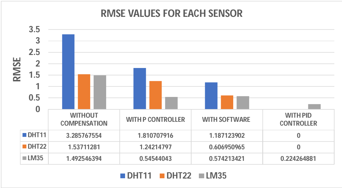
Graph 14: Comparison of RMSE values for DHT11, DHT22, LM35 sensors with and without compensation.
