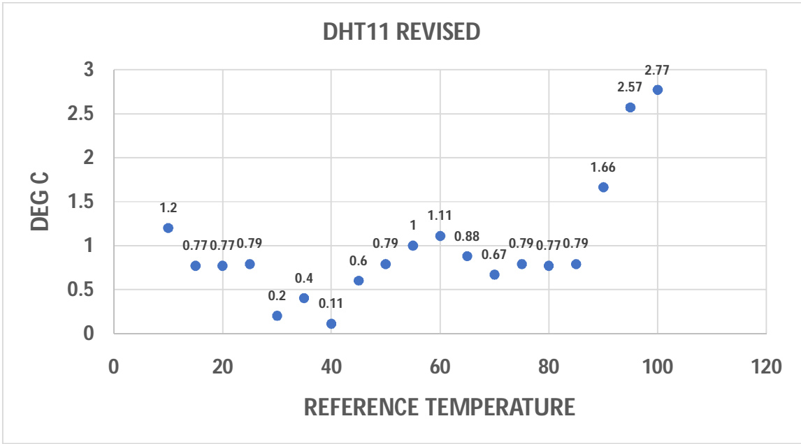
Graph 10: Absolute error of DHT11 with second method.
