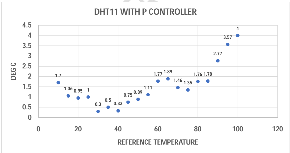
Graph 5: Absolute error of DHT11 with third method
