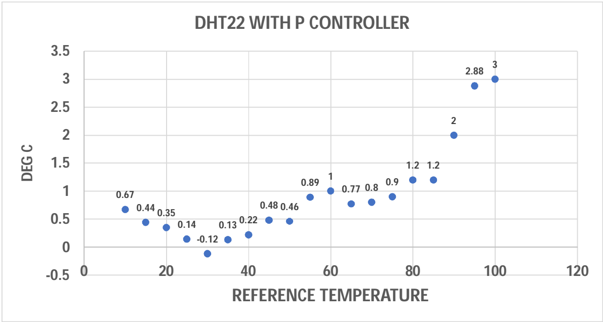
Graph 6: Absolute error of DHT22 with third method
