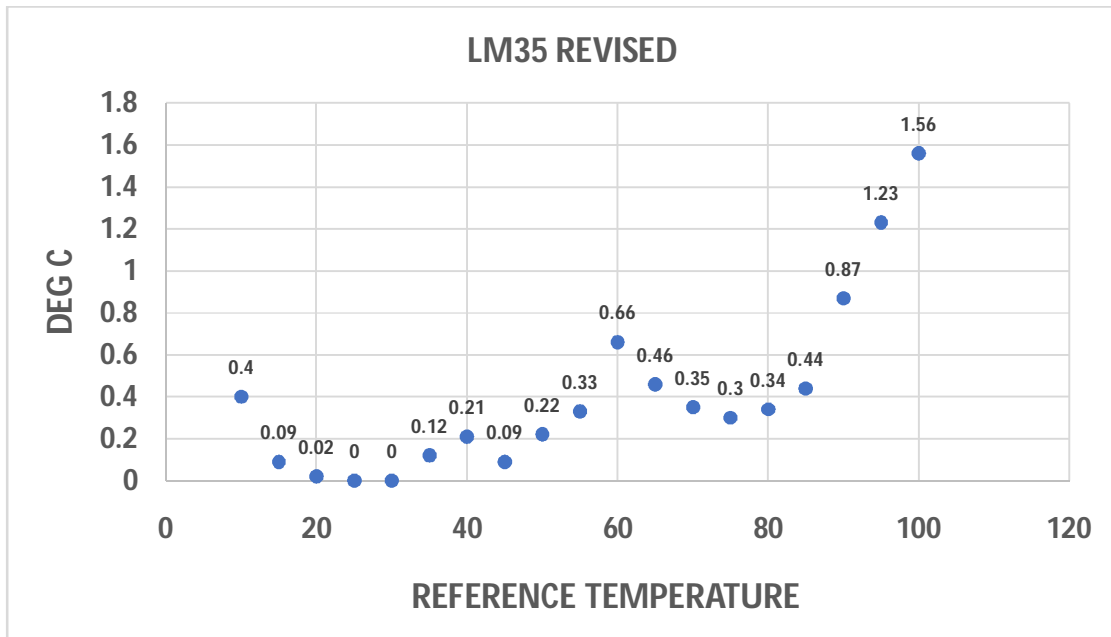
Graph 12: Absolute error of LM35 with second method
