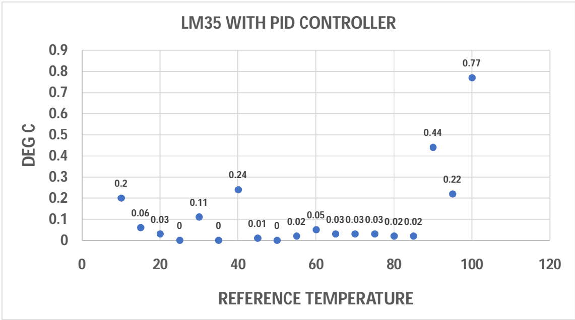
Graph 8: Absolute error of LM35 with PID controller in third method
