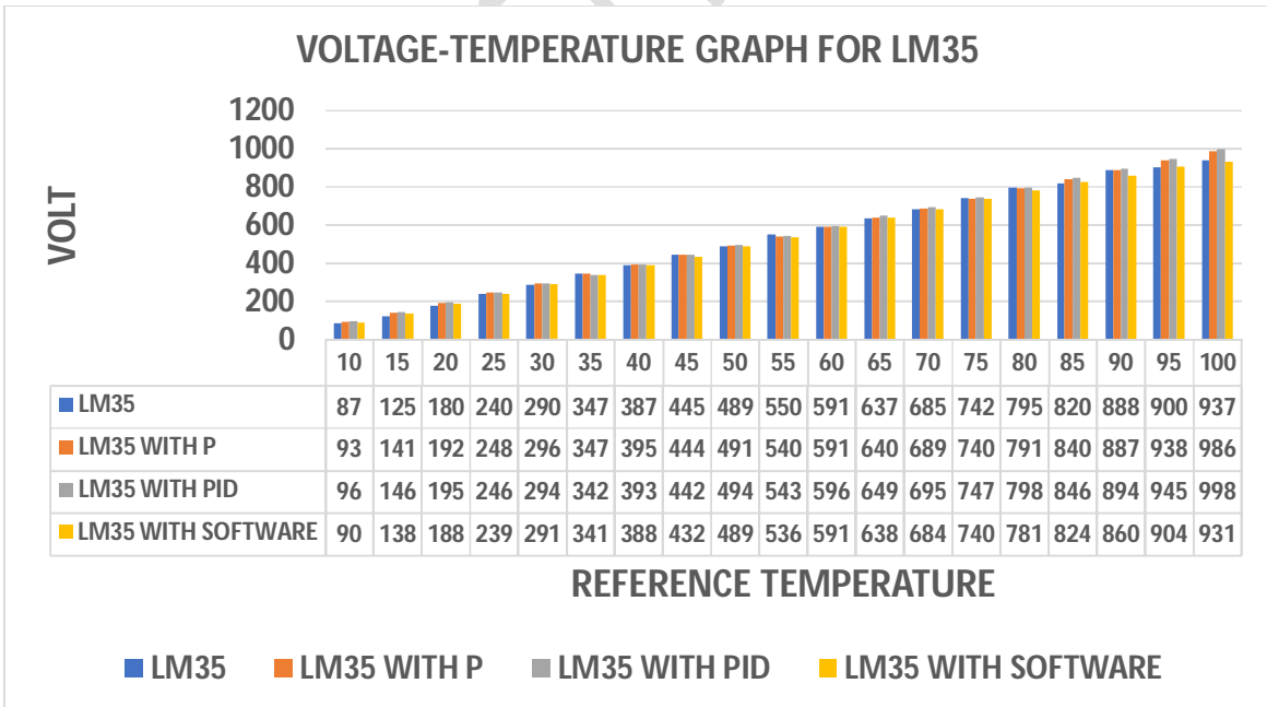
Graph 15: Voltage-Temperature sensitivity plot for LM35 with and without compensation.
