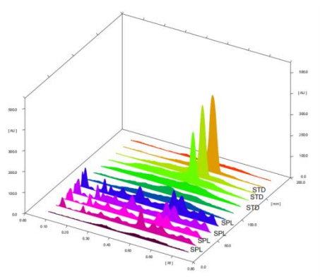
Figure 2. 3D spectra of Ursolic acid + B. racemosa
