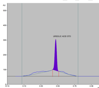
Figure 1a. Typical Chromatogram of standard ursolic acid
