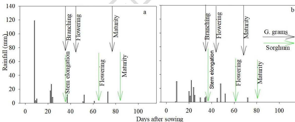
Figure 1. Rainfall (mm) during sorghum and green gram growing period at Mwala (a) and Katangi (b) during the 2022 short rains season
