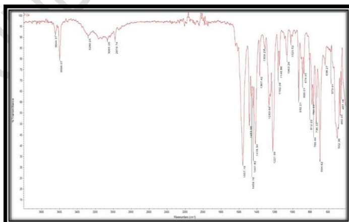
Fig 03. FTIR spectroscopy of Fenopropfen Calcium:
