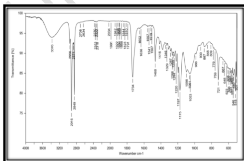
Fig 05. FTIR spectrum of Span 60.
