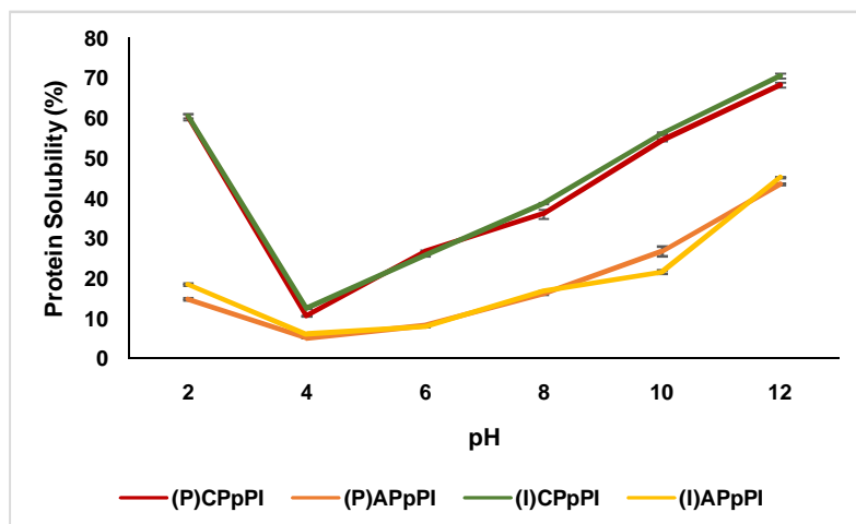
Figure 1. Protein solubility (%) of control and autoclaved PpPI. (P) CPpPI- Control PpPI of Pusa Arhar 2018-4. (P) APpPI- Autoclaved PpPI of Pusa Arhar 2018-4, (I)CPpPI - Control PpPI of ICP 1452, (I)APpPI- Autoclaved PpPI of ICP 1452.
