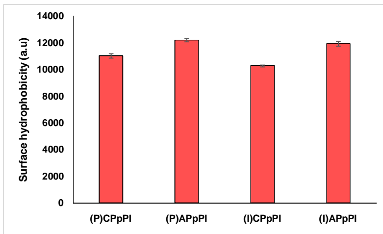
Figure 2. Surface hydrophobicity of control and autoclaved PpPI. (P) CPpPI- Control PpPI of Pusa Arhar 2018-4, (P) APpPI- Autoclaved PpPI of Pusa Arhar 2018-4, (I)CPpPI - Control PpPI of ICP 1452, (I)APpPI- Autoclaved PpPI of ICP 1452.
