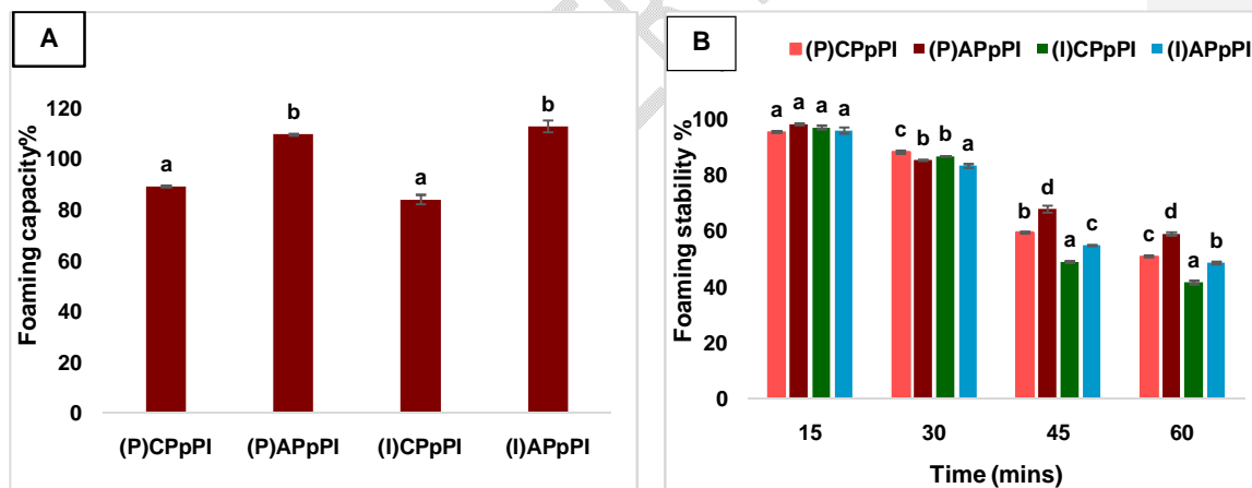
Figure 5. A. Foaming capacity (%) and B. foaming stability (%) of control and autoclaved PpPI. (P) CPpPI- Control PpPI of Pusa Arhar 2018-4, (P)APpPI- Autoclaved PpPI of Pusa Arhar 2018-4, (I)CPpPI - Control PpPI of ICP 1452, (I)APpPI- Autoclaved PpPI of ICP 1452.
