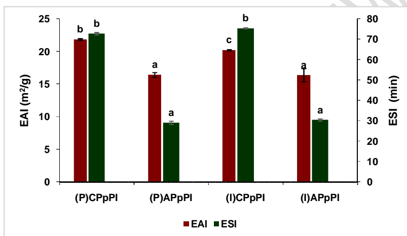
Figure 4. Emulsification ability index (m 2 /g) and emulsification stability index (min) of control and autoclaved PpPI. (P) CpPI- Control PpPI of Pusa Arhar 2018-4, (P) ApPI- Autoclaved PpPI of Pusa Arhar 2018-4, (I)CpPI - Control PpPI of ICP 1452, (I)ApPI- Autoclaved PpPI of ICP 1452.
