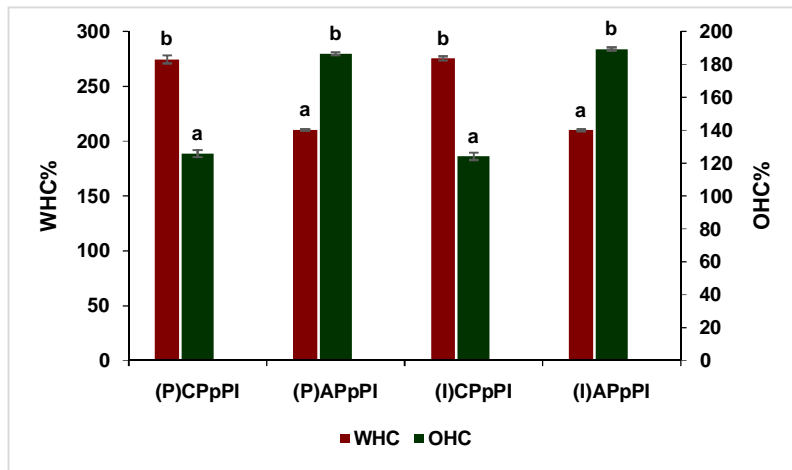
Figure 3. Water holding capacity (%) and oil holding capacity (%) of control and autoclaved PpPI. (P) CPpPI- Control PpPI of Pusa Arhar 2018-4, (P) APpPI- Autoclaved PpPI of Pusa Arhar 2018-4, (I)CPpPI - Control PpPI of ICP 1452, (I)APpPI- Autoclaved PpPI of ICP 1452
