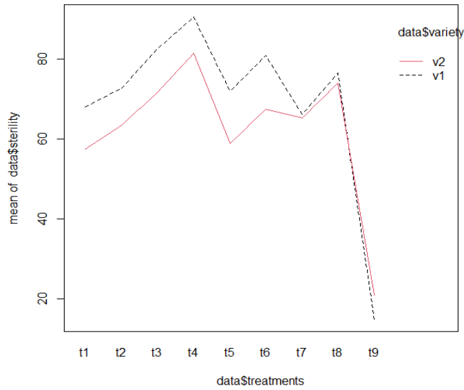
Fig 6: Comparison of pollen sterility recorded in different treatments between two varieties
