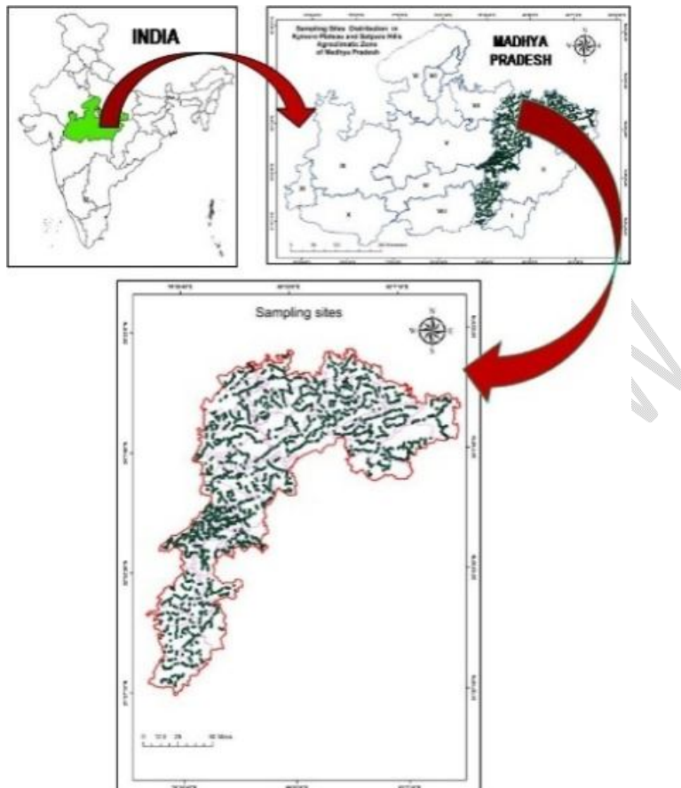
Figure 1: Sampling sites in the study area
