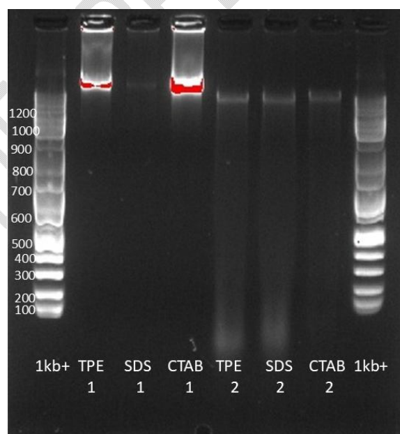
Figure 2. Gel visualization
