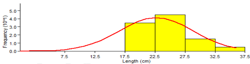
Fig (1). total length frequency distribution of S. schall from Upper Atbara and Setit complex dam.
