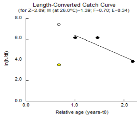
Fig. (4). Total, natural, and fishing mortality using length-converted catch curve from FISAT output.
