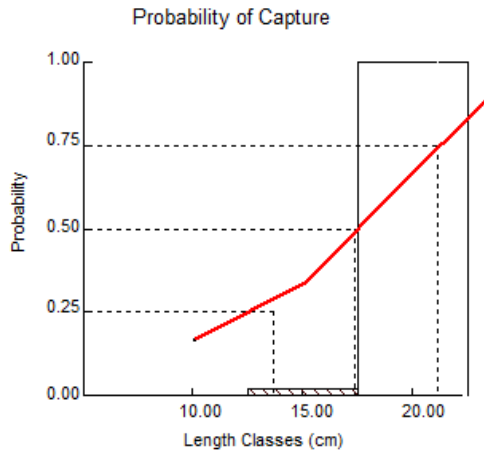
Fig. (6). Capture probability of S. shall .
