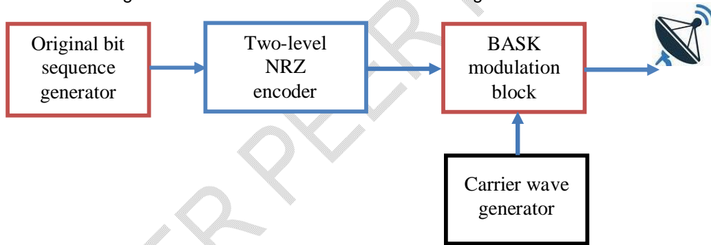
Fig.5. Structure Diagram of the BASK Modulator
