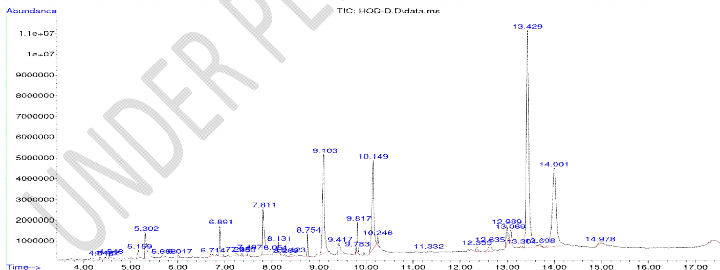
Figure2: GC-MS Spectra (Chromatogram) of Dichloromethane extract fraction of Rauwolfia vomitoria
